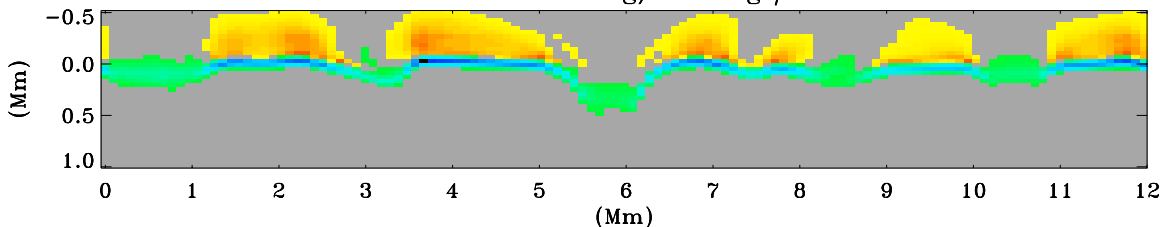
Radiative Heating/Cooling \mu = \pm 0.5
