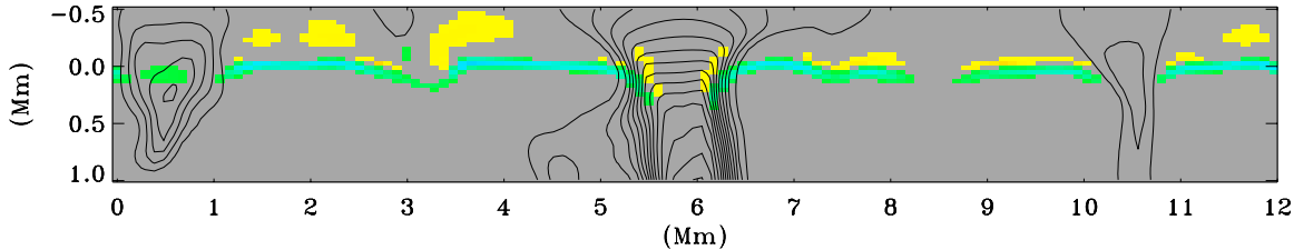
Radiative Heating/Cooling \mu = \pm 1
