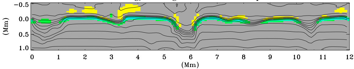
Net Radiative Heating/Cooling with 250 G B-Field Contours
