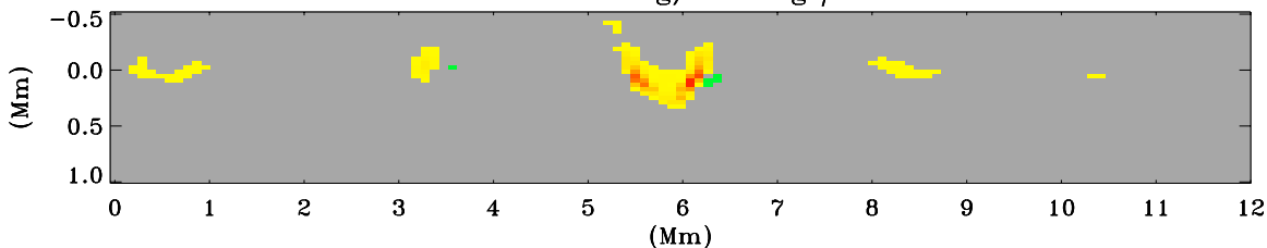
Radiative Heating/Cooling \mu = \pm 0.05
